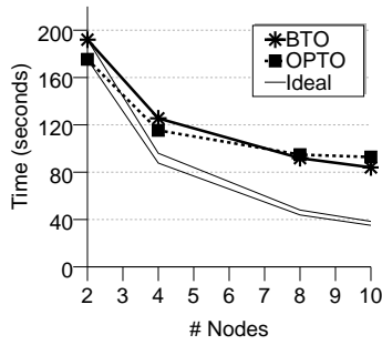
(a) Stage 1 (token ordering).
